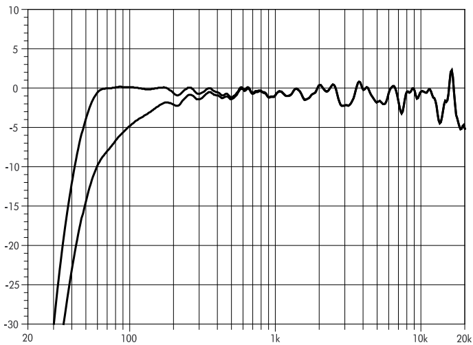
Fig. 18: 12S-D frequency response, standard and CUT modes
