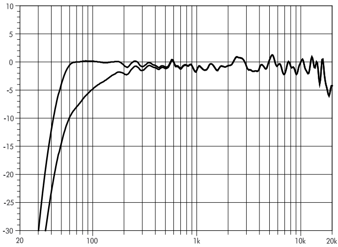
Fig. 17: 12S frequency response, standard and CUT modes
