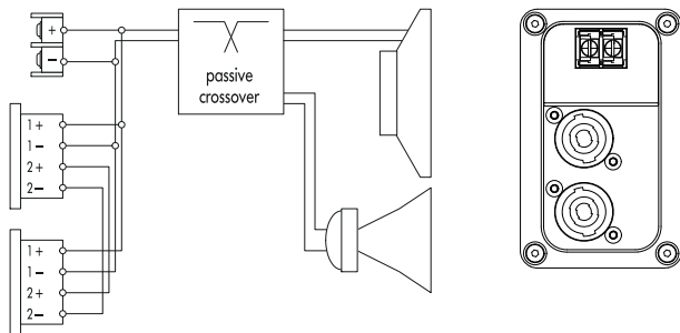
Fig. 2: Connector wiring
