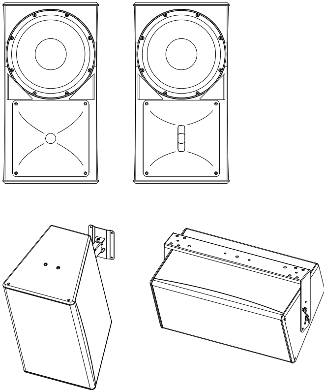
Fig. 1: 12S/12S-D loudspeaker
